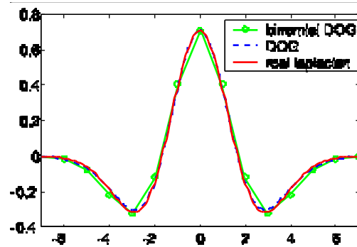
Figure 5: Comparisons of real Laplacian versus real DoG and binomial DoG for \sigma_{dog} = \sqrt{2} and \sigma_1 = \sqrt{2} \sigma_{dog} and \sigma_{lap} = 1.7
